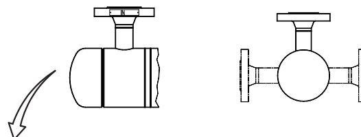
Alternative steam inlets
